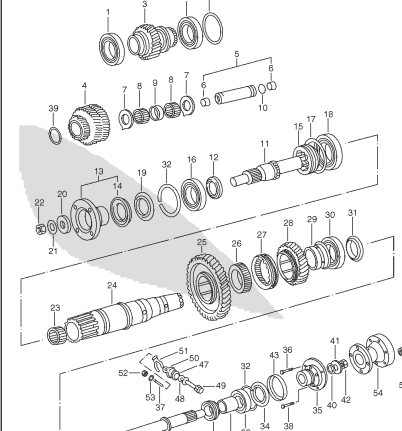
FIG. 49 TRANSFER GEAR
