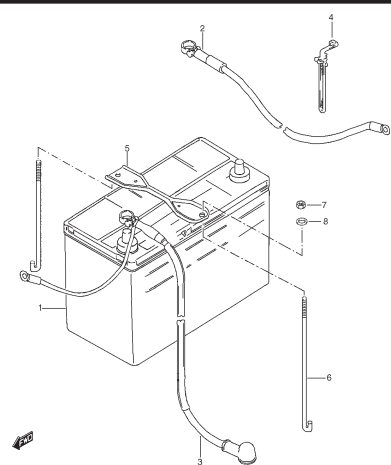
FIG. 55 BATTERY
