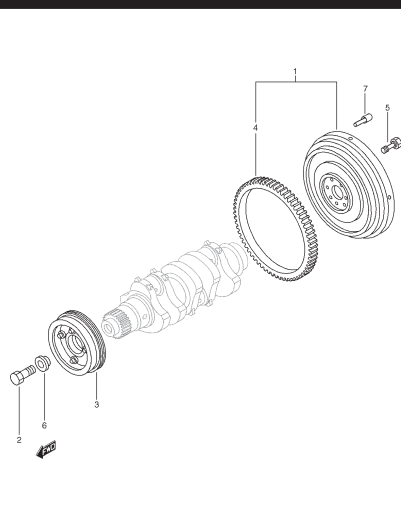
FIG. 13 ENGINE FLYWHEEL
