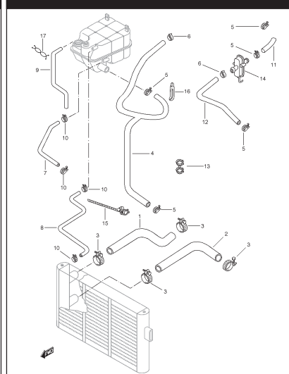
FIG. 38 WATER NOSE
