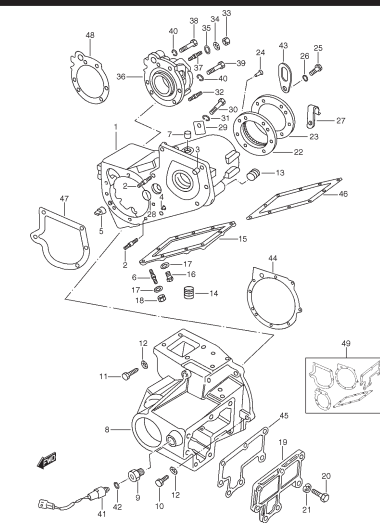
FIG. 51 TRANSFER CASE
