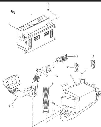
FIG. 99 INTERIOR TRIM
