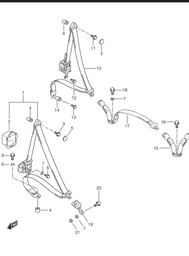
FIG. 115 SEAT BELT
