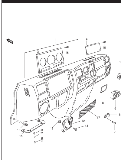
FIG. 94 INSTRUMENT PANEL
