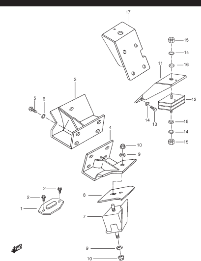
FIG. 36 ENGINE MOUNTING
