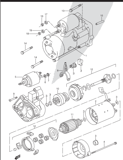
FIG. 53 STARTING MOTOR
