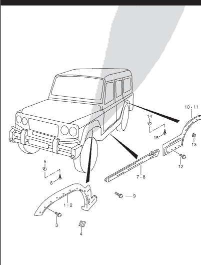
FIG. 101 GARNISH / SPLASH GUARD
