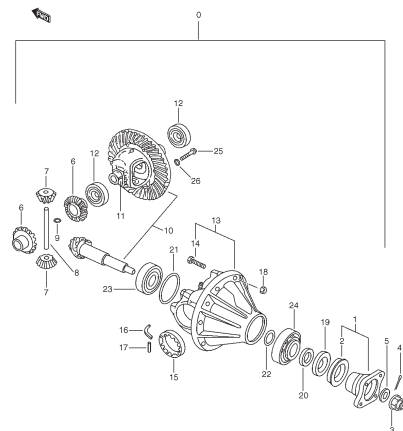
FIG. 47 FRONT DIFF GEAR
