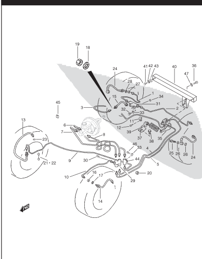
FIG. 76 BRAKE PIPING
