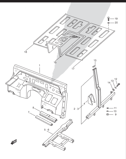
FIG. 85 FRONT BODY
