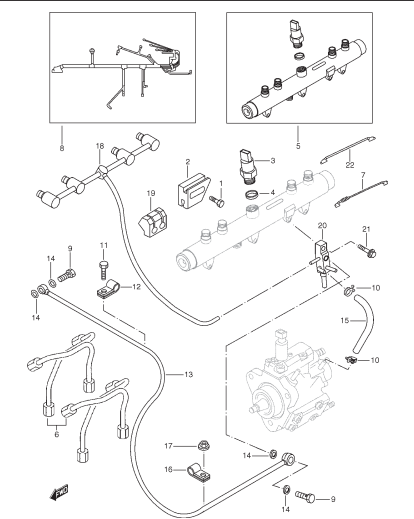
FIG. 20A INJECTION PIPING (TYPE 2)
