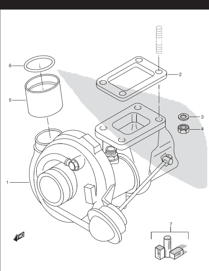
FIG. 21 TURBOCHARGER
