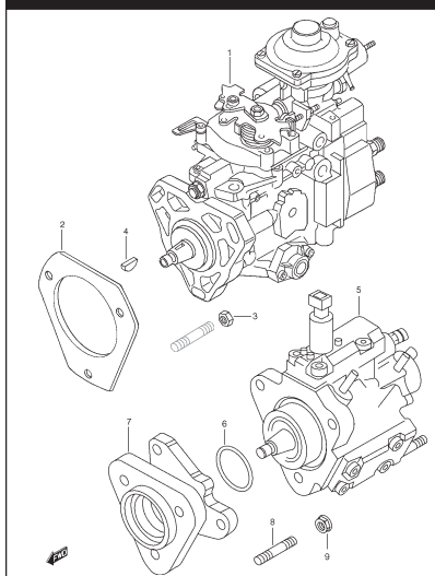
FIG. 16 INJECTION PUMP
