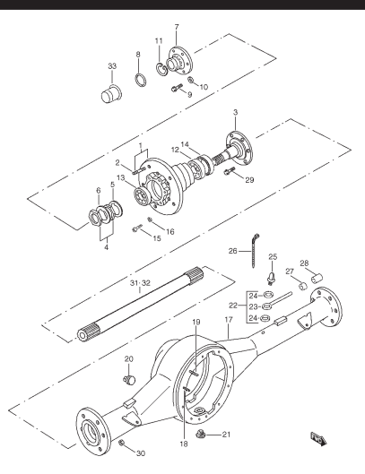
FIG. 67 REAR AXLE
