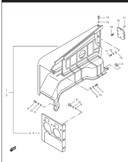
FIG. 83 FRONT FENDERS
