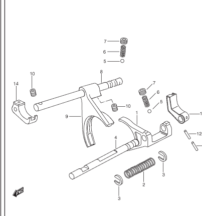
FIG. 50 TRANSFER GEAR SHIFTING
