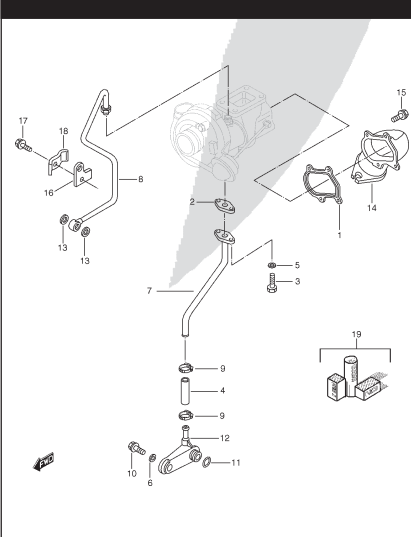
FIG. 22 SUPERCHARGING LINES
