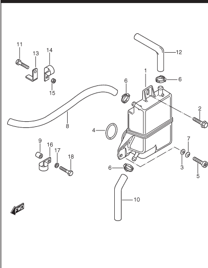
FIG. 5 ENGINE BREATHER
