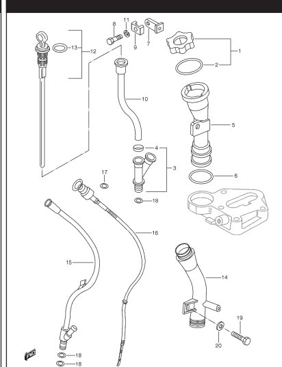
FIG. 23 OIL DIPSTICK
