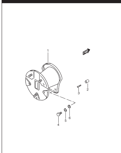
FIG. 102 SPARE TIRE
