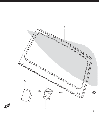
FIG. 84 WINDSHIELD GLASS
