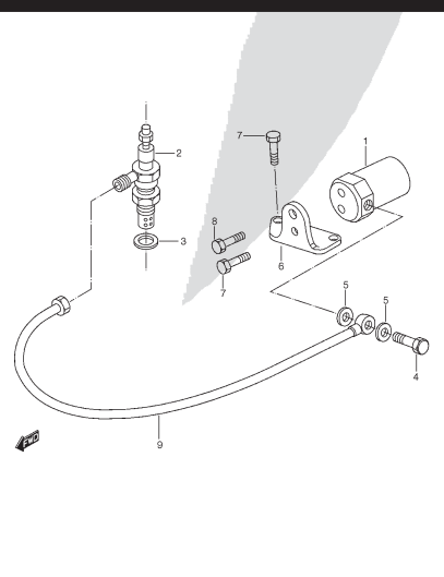
FIG. 30 PRE-HEATING SYSTEM
