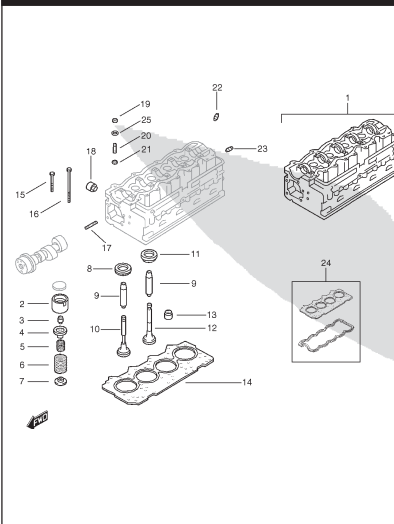
FIG. 6 CYLINDER HEAD
