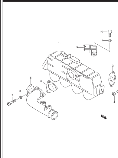
FIG. 8 INTAKE MANIFOLD
