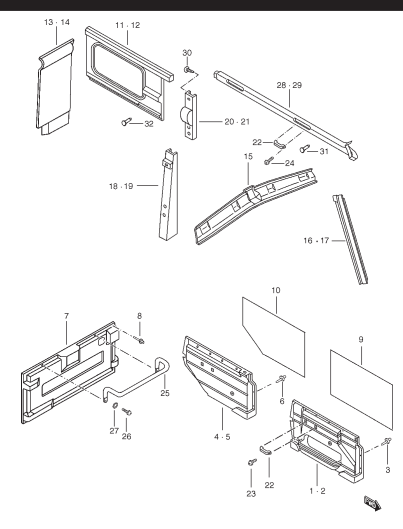
FIG. 99 INTERIOR TRIM
