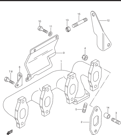
FIG. 9 EXHAUST MANIFOLD
