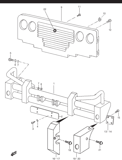
FIG. 91 FRONT BUMPER & GRILLE
