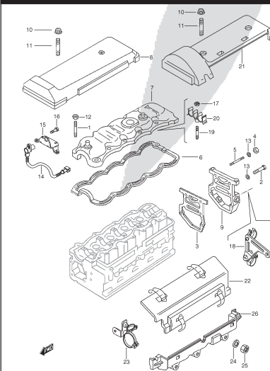
FIG. 7 CYLINDER HEAD COVER
